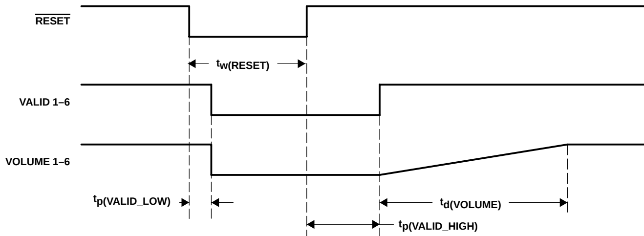
Figure 5–1. \overline{\text{RESET}} Timing
